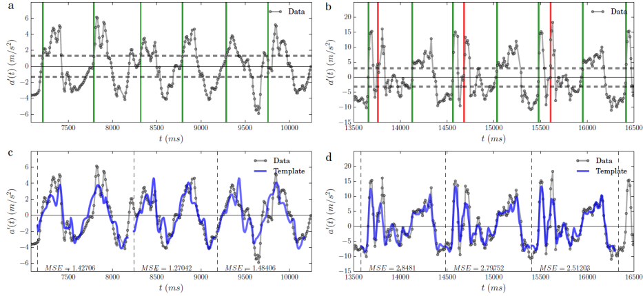
Fig. 2. Counting steps with the threshold and template approaches. In a and b, the lower and upper threshold are shown in the horizontal, dashed grey lines. The vertical lines represent the estimated start of each step, where green indicates correct registrations and red incorrect steps. In c and d the template method is used on the same signals, where the template (in blue) is matched to the signal in intervals demarcated by dashed vertical lines.
